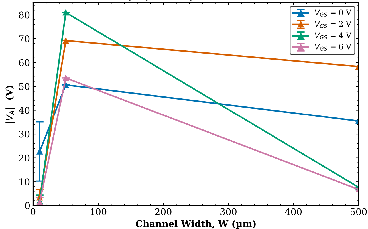
TFT2 Combined (Tr. 1 & 2) |V_A| vs W | L = 40\text{ }\mu\text{m}
